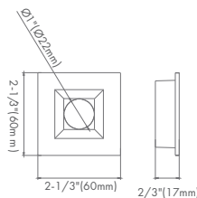
1" SQUARE TRIM
